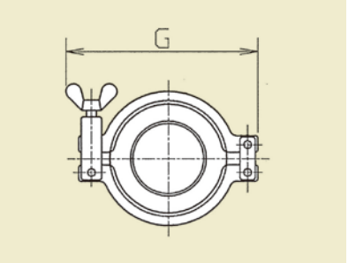
CLAMP BANDS
